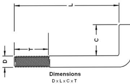
Anchor Bolt (Right Angle Bend)
