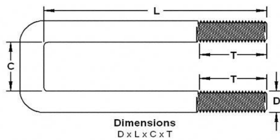
U-Bolts (Square Bend)
